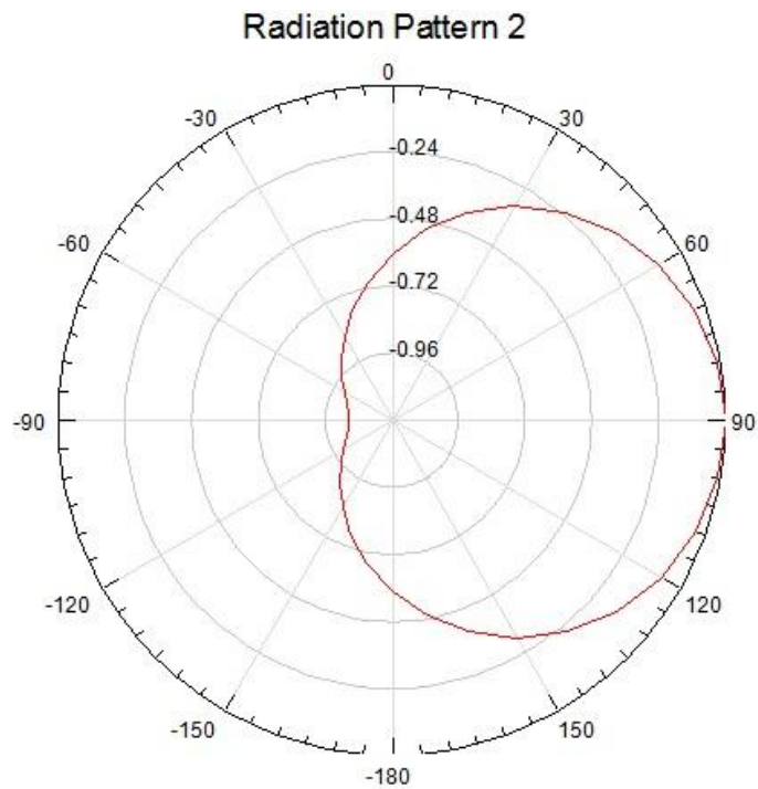
(Relative Read Range vs. Orientation)
